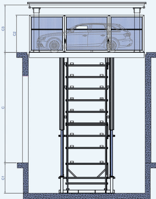
Section View-UP
