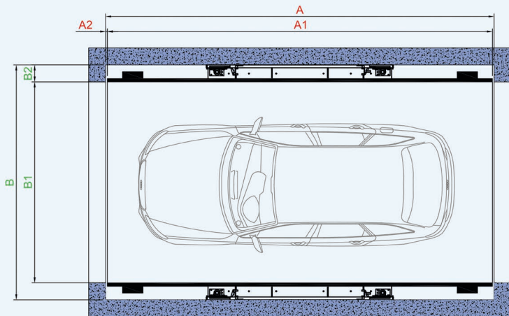
Section View-DOWN
