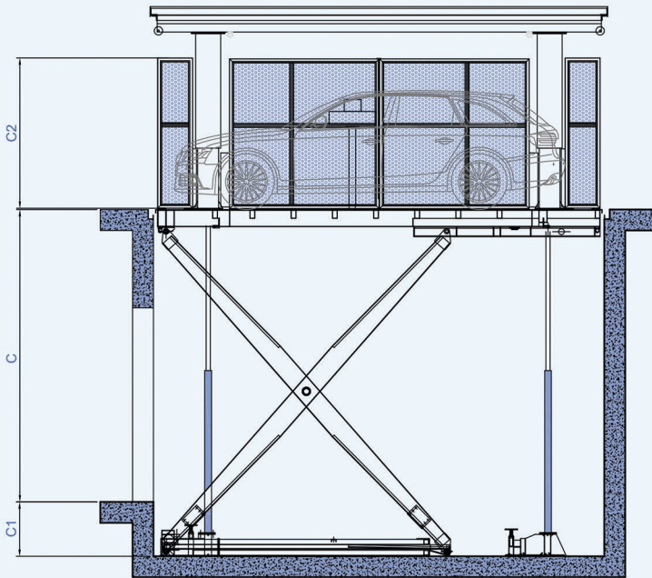
Section View-UP
