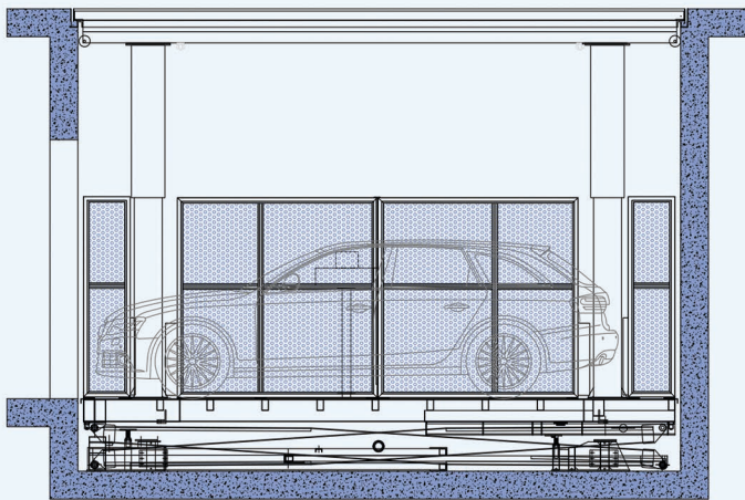
Section View-DOWN
